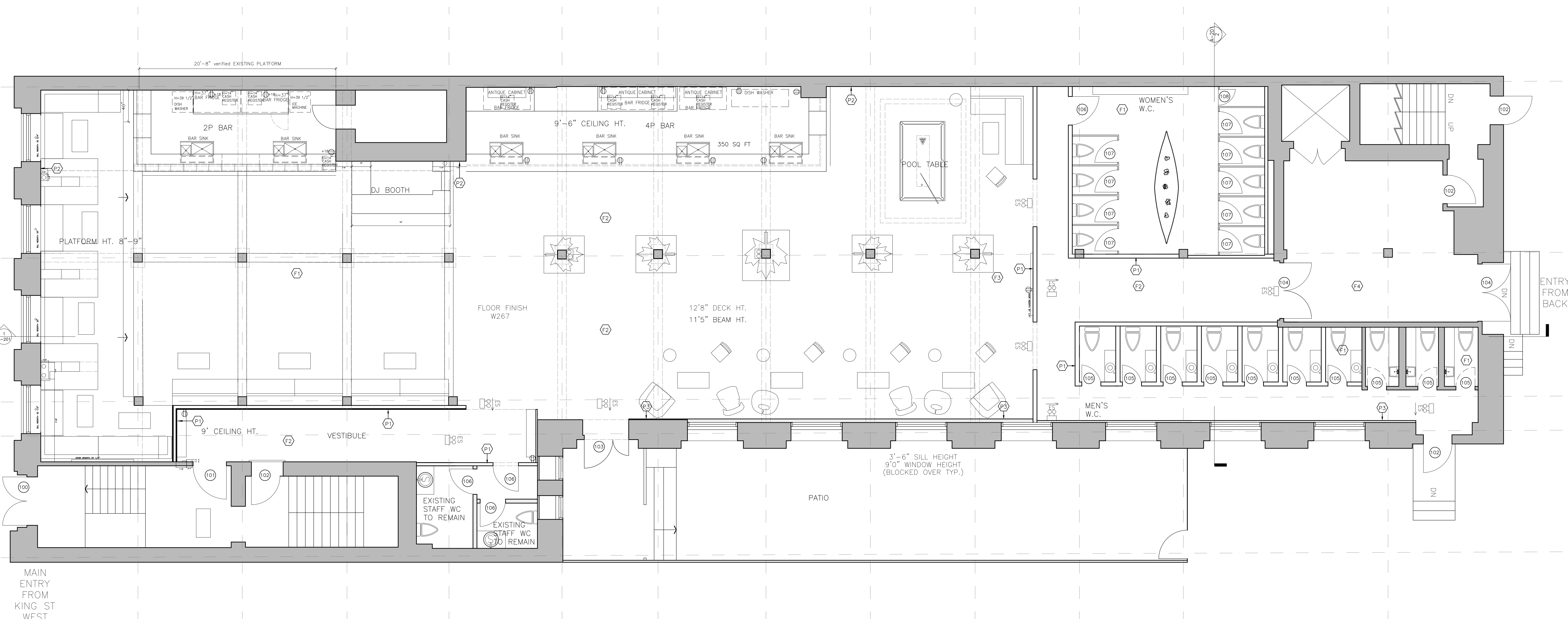
1 PROPOSED GROUND FLOOR PLAN A-102
